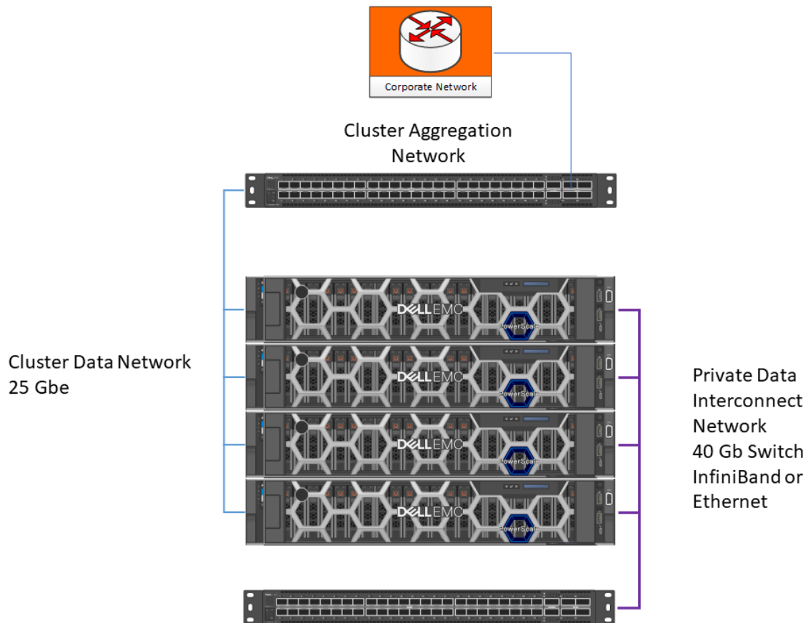
Figure 7. PowerScale networking
