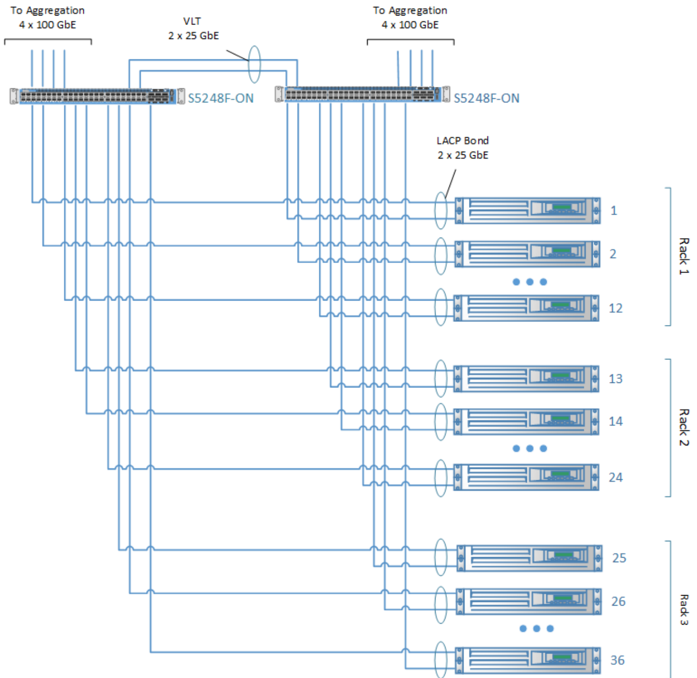
Figure 4. 25 GbE single pod networking equipment
