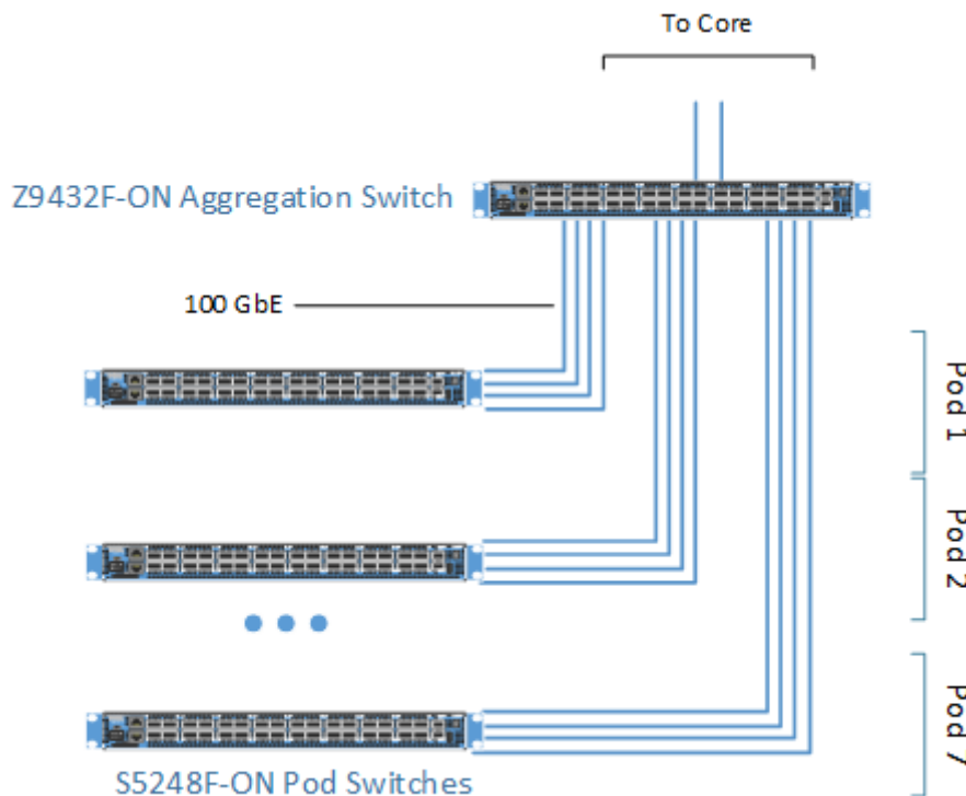
Figure 5. Multiple pod networking equipment
