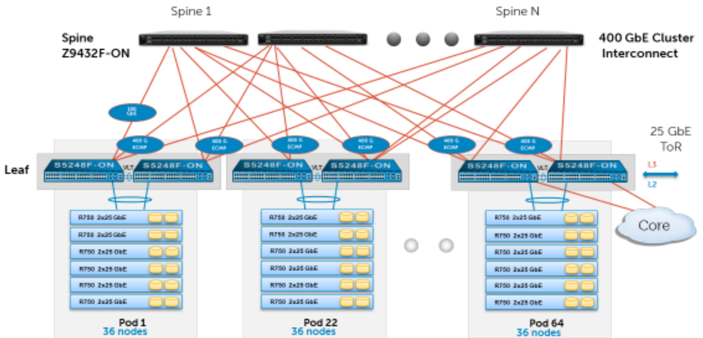
Figure 6. Multiple pod view with Layer 3 ECMP
